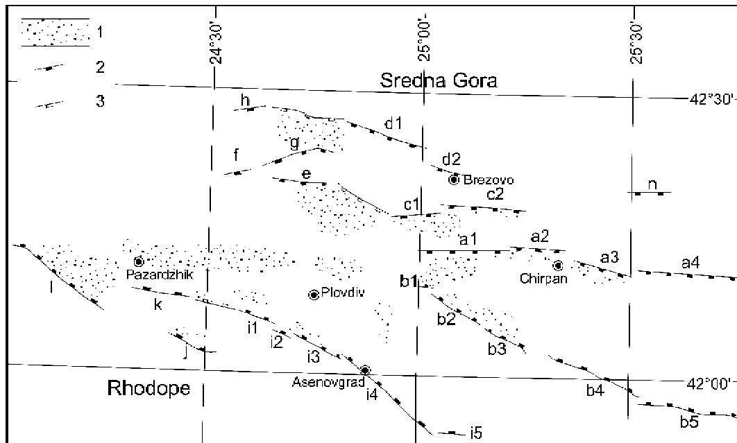
Fig. 2. Geometric fault segments in the Plovdiv Depression. Geometric fault segments labeled by letters or letters and numbers. 1 – Quaternary depocentre; 2 – geometric fault segment based on fault scarps; 3 – fault segment assumed from Quaternary hanging wall basin. Projection is UTM Zone 35, Northern Hemisphere
