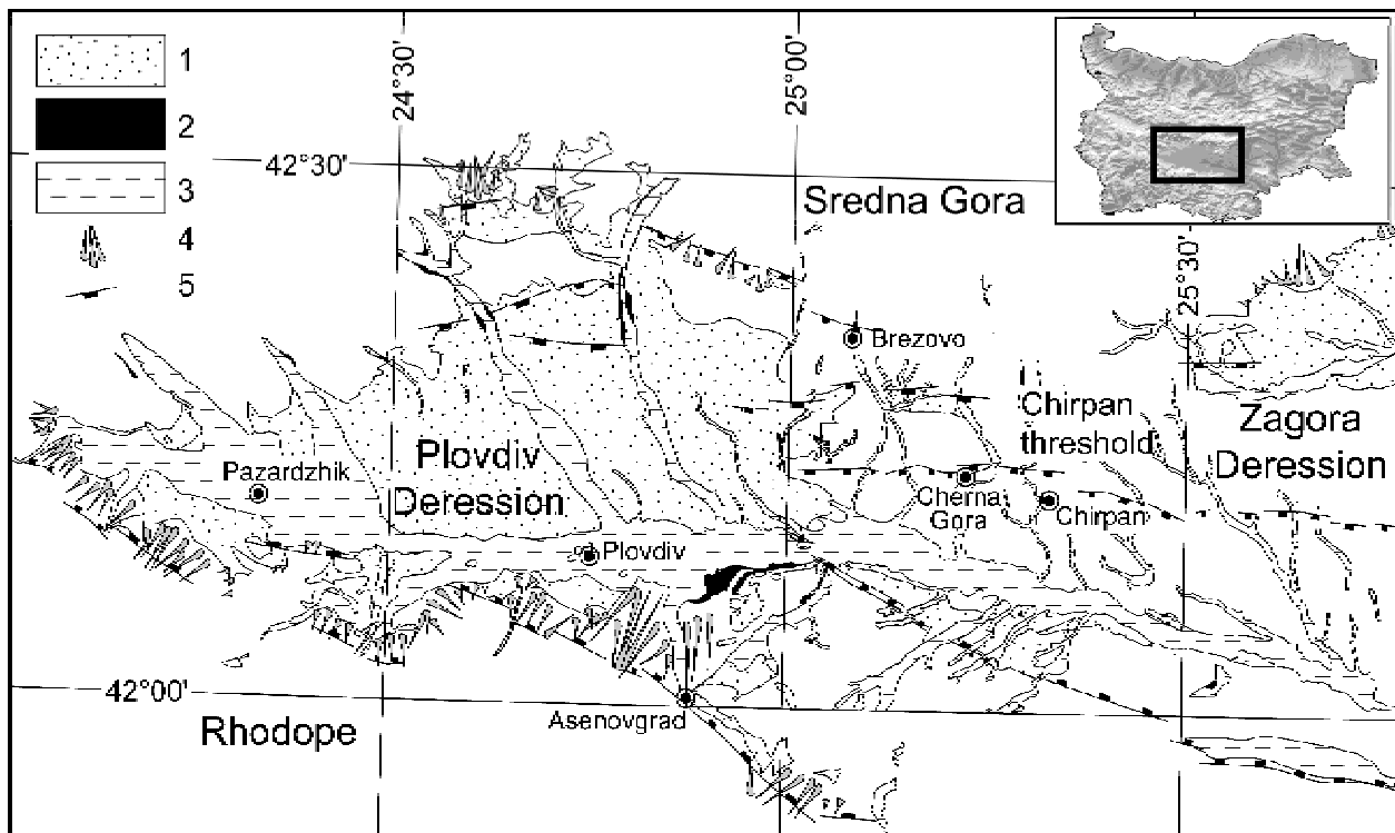
Fig. 1. Quaternary sediments (from Geological map of Bulgaria 1:100 000 scale) and fault scarps in the Plovdiv Depression. 1 – Quaternary mainly alluvial sediment; 2 – Late Pleistocene river terrace in fault footwalls; 3 – Holocene floodplain; 4 – alluvial fan; 5 – fault scarp. Projection is UTM Zone 35, Northern Hemisphere
